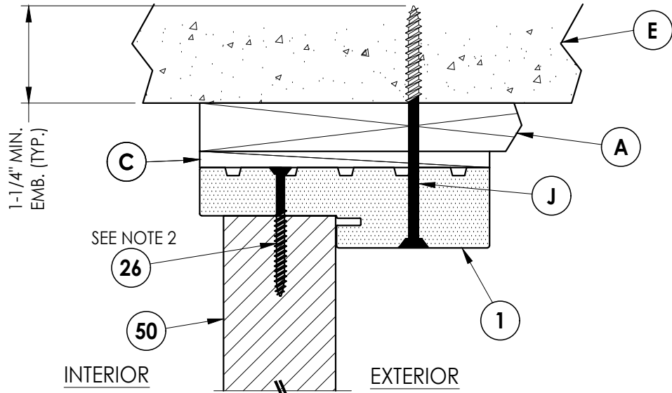
4 7 VERTICAL CROSS SECTION Shown w/ 1X sub-buck Inswing shown (Outswing similar)
