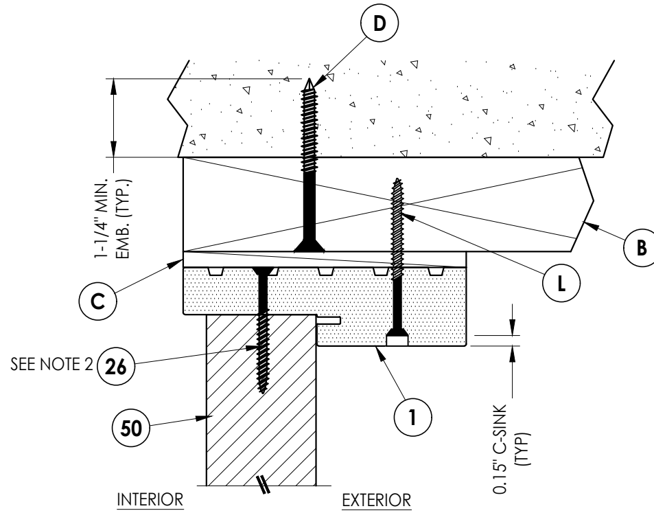
4 6 VERTICAL CROSS SECTION Shown w/ 2X Buck Inswing shown (Outswing similar)
