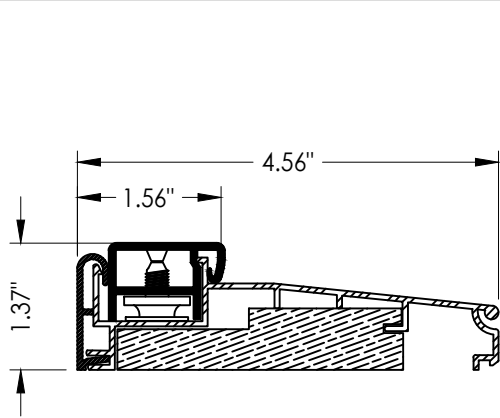
13 INSWING THRESHOLD WORLDWIDE
