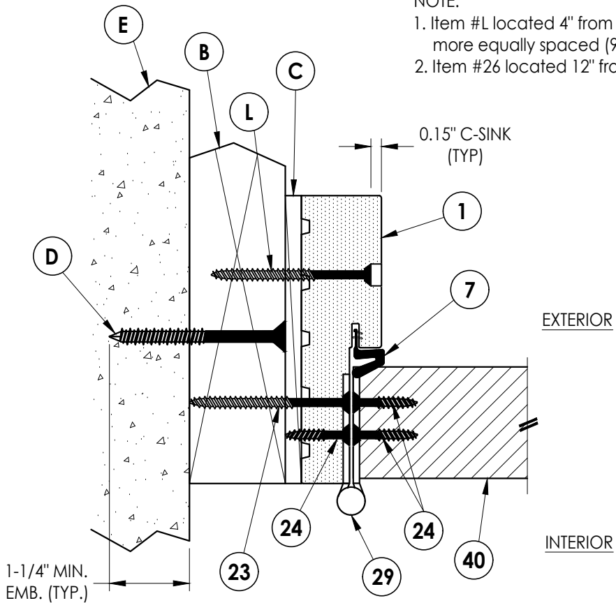
1 6 HORIZONTAL CROSS SECTION Shown w/ 2X Buck Inswing shown (Outswing similar)
