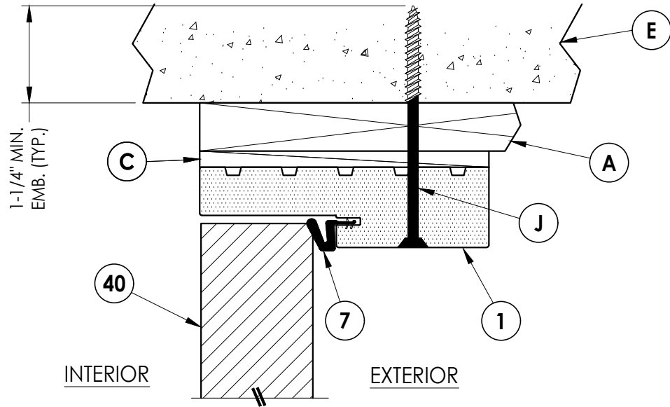
3 7 VERTICAL CROSS SECTION Shown w/ 1X sub-buck Inswing shown (Outswing similar)
