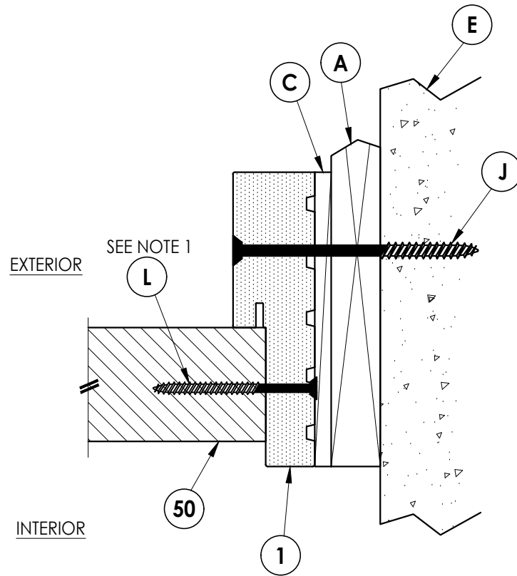
2 7 HORIZONTAL CROSS SECTION Shown w/ 1X sub-buck Inswing shown (Outswing similar)
