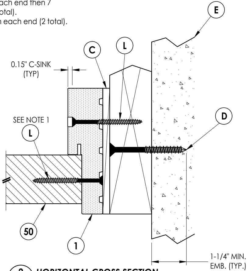
2 6 HORIZONTAL CROSS SECTION Shown w/ 2X Buck Inswing shown (Outswing similar)
