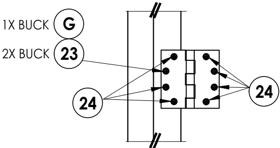
HINGE DETAIL
